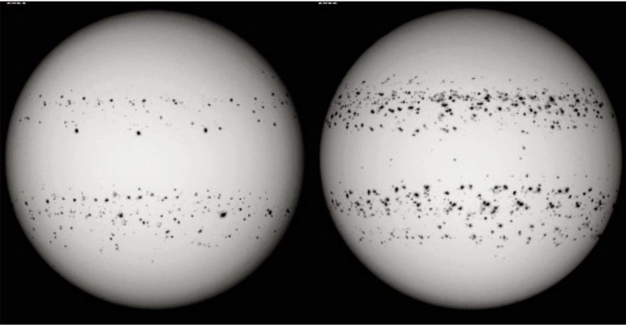
More from spaceweather.com : This image, taken in false color to emphasize the spots, was compiled by Spanish amateur astronomer, Patricio Leon Manchac . It compares solar photos taken in 2021 (left side), vs 2022 (right) then superimposed. The interesting banding of the spots, and what must be an electromagnetic activity at those solar latitudes, could stand more explanation, as do the blank areas. But not in this issue. Meanwhile, I’d say that Sun cycle # 25 is kicking up. ◇
